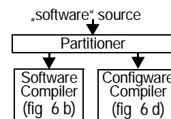
Fig. 14. Software / Configware-Co-Compiler
