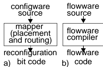
Fig. 4: Separate compilers.
