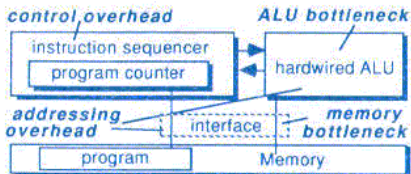
Fig. 1. computers and their von-Neumann bottlenecks
